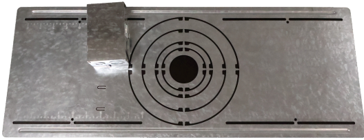
Mounting Plate With Junction Box 2"/3"/4"/6"/8"
