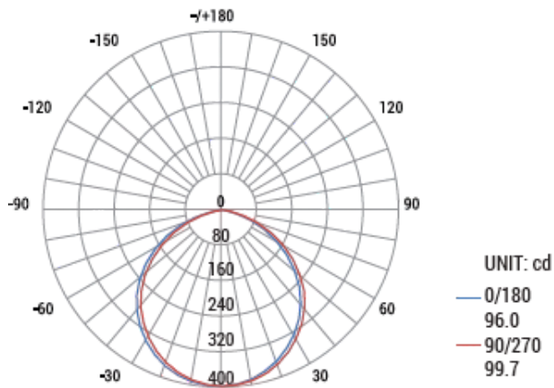
4" Square Retrofit Downlight
