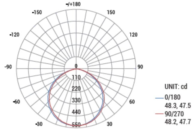
6" Square Retrofit Downlight
