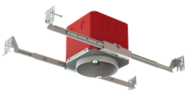
MF4 (4" Fire Resistant Junction Box)
