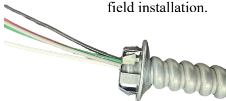
Snap-in head type adapter for easy field installation.
